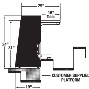
Convertible Tables in Bleachers
