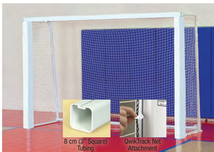
SCFUTSAL Shown with Optional SC03PP Safety Padding
