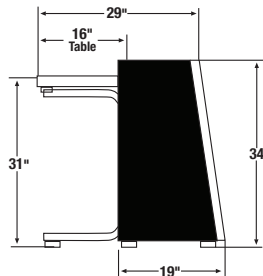
Convertible Tables on Floor
